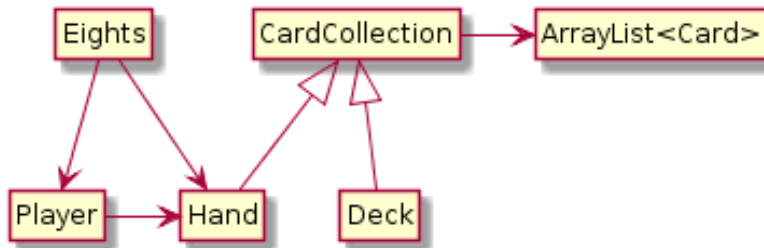
Figure 14.1: UML diagram for the classes in this chapter.
