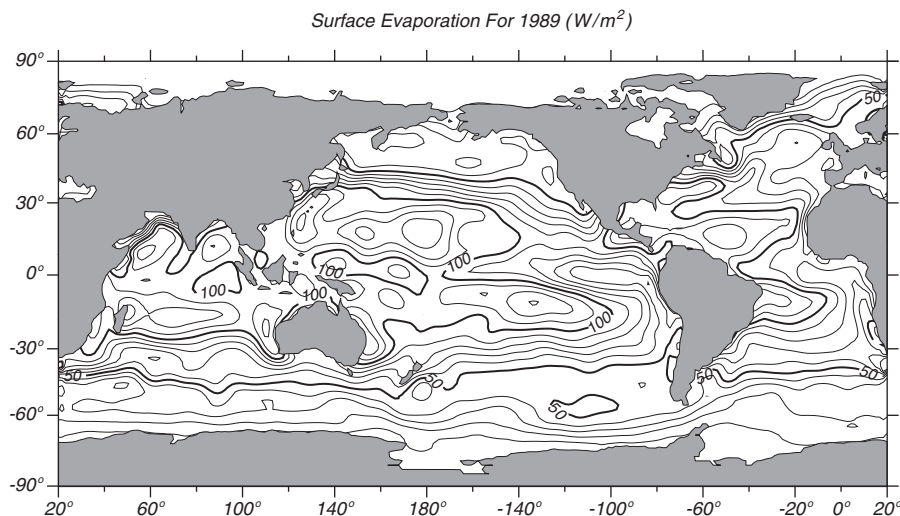
Figure 5.9 Annual-mean latent heat flux from the sea surface Q_L in W/m^2 during 1989 calculated from data compiled by the Data Assimilation Office of NASA's Goddard Space Flight Center using reanalyzed data from the ECMWF numerical weather prediction model. Contour interval is 10 W/m^2 .
