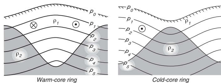
Figure 10.12 Shape of constant-pressure surfaces p_i and the interface between two water masses of density \rho_1, \rho_2 if the upper is rotating faster than the lower. Left: Anticyclonic motion, warm-core eddy. Right: Cyclonic, cold-core eddy. Note that the sea surface p_0 slopes up toward the center of the warm-core ring, and the constant-density surfaces slope down toward the center. Circle with dot is current toward the reader, circle with cross is current away from the reader. After Defant (1961: 466).
