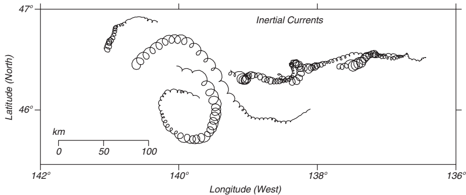
Figure 9.1 Inertial currents in the North Pacific in October 1987 (days 275–300) measured by hole-sock drifting buoys drogued at a depth of 15 meters. Positions were observed 10–12 times per day by the Argos system on NOAA polar-orbiting weather satellites and interpolated to positions every three hours. The largest currents were generated by a storm on day 277. Note these are not individual eddies. The entire surface is rotating. A drogue placed anywhere in the region would have the same circular motion. After van Meurs (1998).
