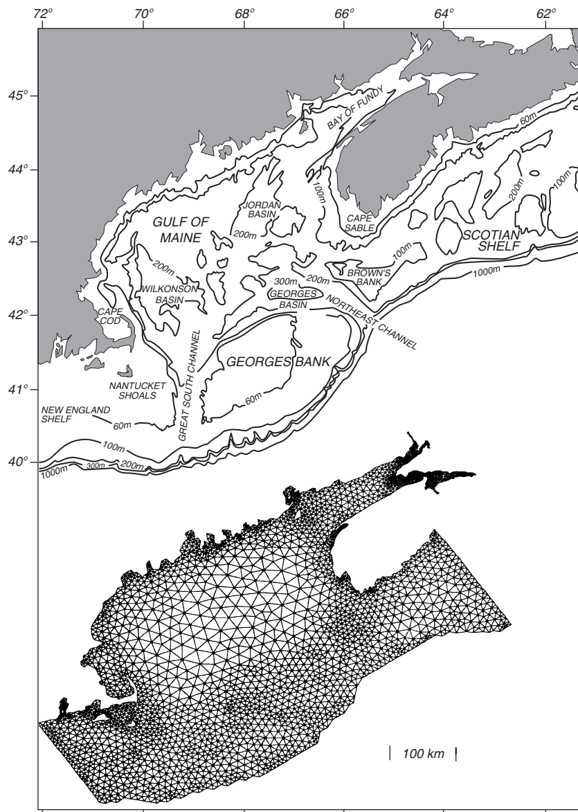
Figure 15.3 Top : Topographic map of the Gulf of Maine showing important features. Inset : Triangular, finite-element grid used to compute flow in the gulf. The size of the triangles varies with depth and rate of change of depth. After Lynch et al, (1996).
