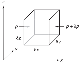
Figure 7.3 Sketch of flow used for deriving the pressure term in the momentum equation.
