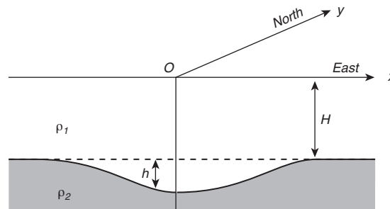
Figure 14.9 Sketch of the two-layer model of the equatorial ocean used to calculate planetary waves in those regions. After Philander (1990: 107).
