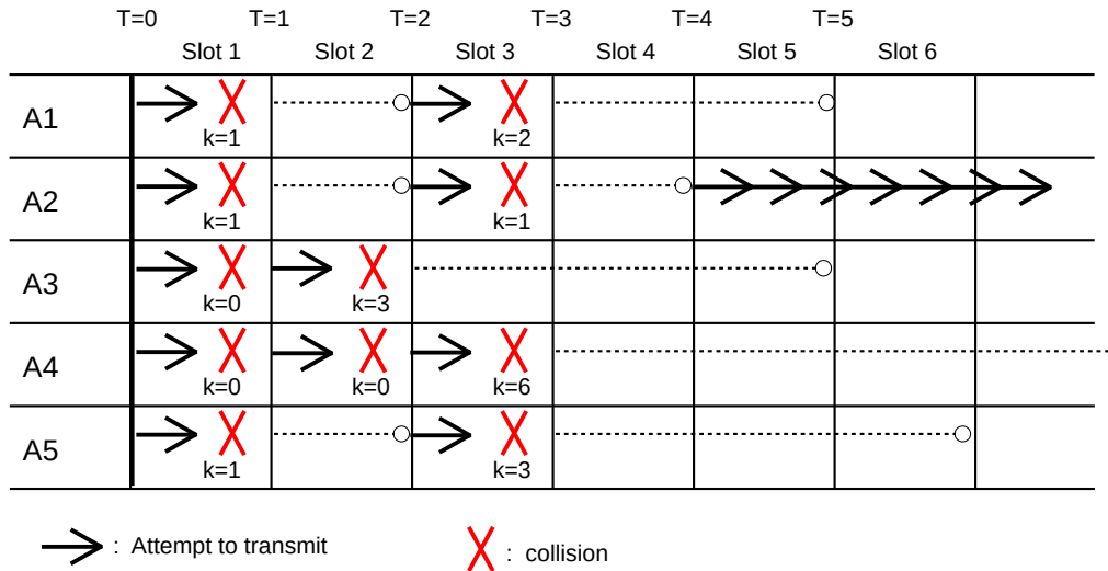
Fig. 11:: Ethernet collisions with exponential backoff
