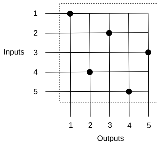
Fig. 17:: 5×5 crossbar with 5 parallel connections 1→1, 2→3, 3→5, 4→2, 5→4
