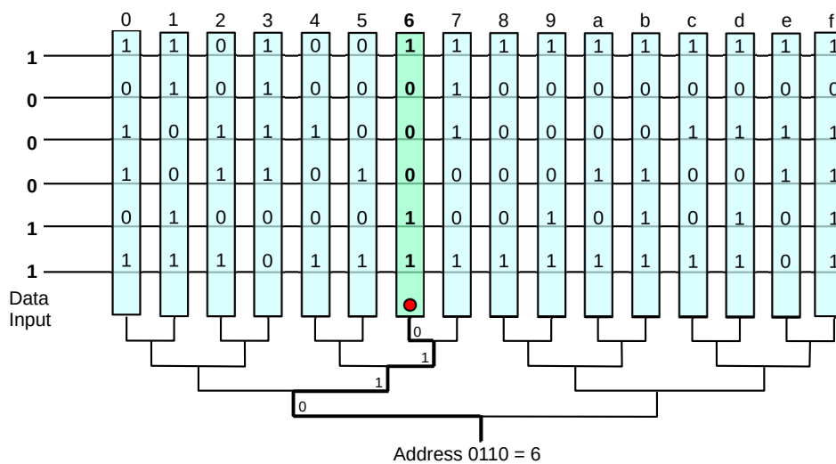
Fig. 18:: Content-Addressable Memory
