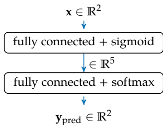
Figure D.4. A simple, two-layer, fully connected network trained to classify whether a given coordinate lies within a circle (shown in white). The nonlinearities allow neural networks to form complicated, nonlinear decision boundaries.
