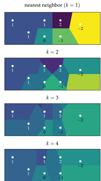
Figure 8.1. Approximating the values of states in a two-dimensional, continuous state space using the mean of the utility values of their k -nearest neighbors according to Euclidean distance. The resulting value function is piecewise constant.
