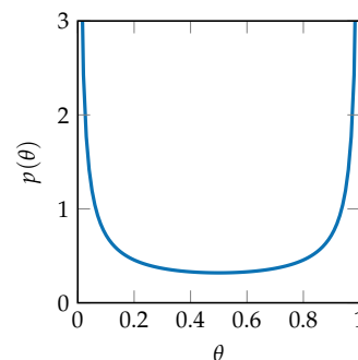
Figure 4.2. An example of a distribution where the expected value of \theta is not a good estimate. The expected value of 0.5 has a lower density than occurs at the extreme values of 0 or 1. This distribution happens to be a beta distribution, a type of distribution we will discuss shortly, with parameters (0.2, 0.2).
