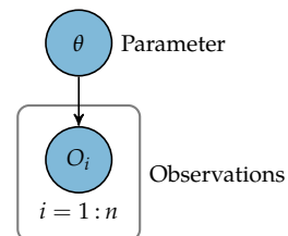
Figure 4.3. Bayesian network representing parameter learning.
