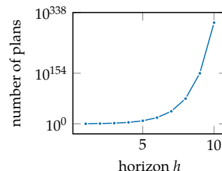
Figure 20.2. Even for small POMDPs with only two actions and two observations, the number of possible plans grows extremely quickly with the planning horizon. We can often significantly prune the set of alpha vectors at each iteration and only consider far fewer plans.
