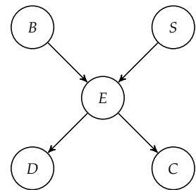
Figure 3.1. Bayesian network structure from example 2.5.
