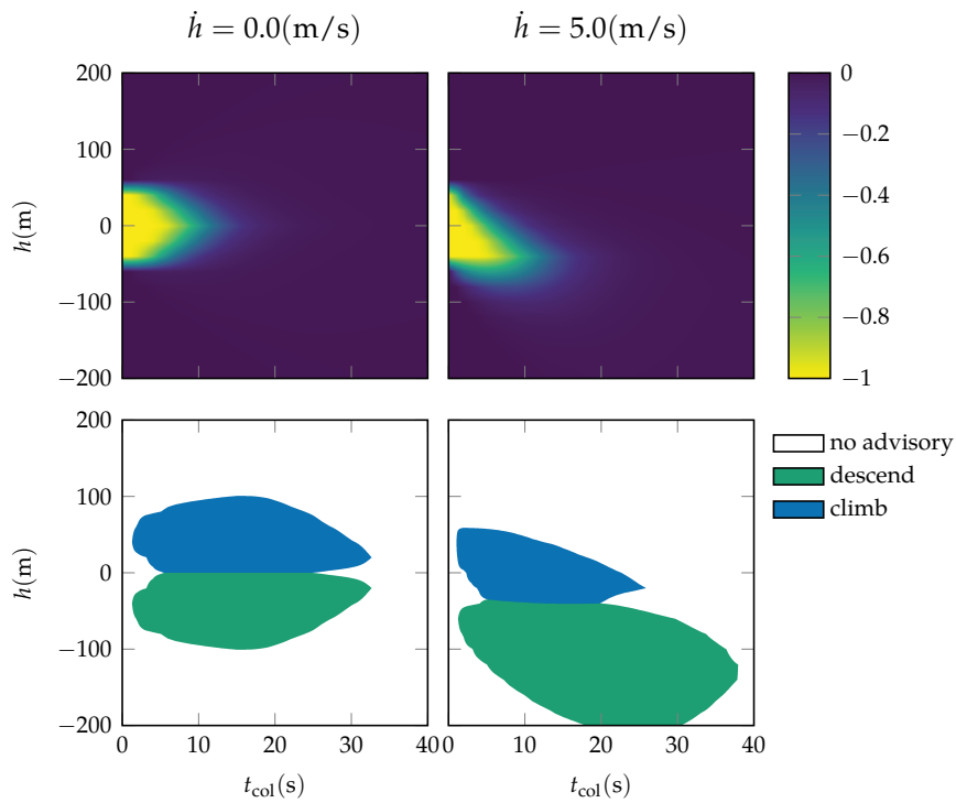
Figure F.9. Optimal value function slices (top) and policy slices (bottom) for the aircraft collision avoidance problem. The value function and policy are symmetric about 0 when the vertical separation rate is 0, but are skewed when the vertical separation rate is nonzero. Overall, our aircraft need not take action until the intruder aircraft is close.
