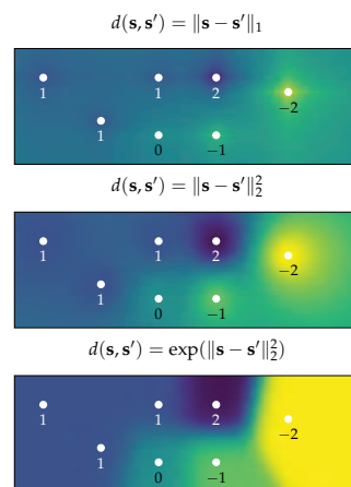
Figure 8.2. Approximating the values of states in a two-dimensional continuous state space by assigning values based on proximity to several states with known values. Approximations are constructed using several distance functions.
