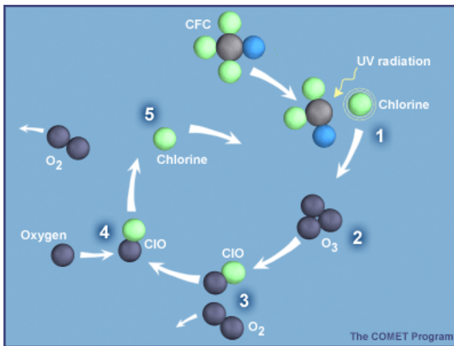
Figure 3. CFCs destroy ozone ( O_3 ) when a chlorine atom breaks loose from the CFC and interacts with the oxygen atoms in the ozone molecule. This Photo by UCAR is licensed under CC BY-SA-NC .
