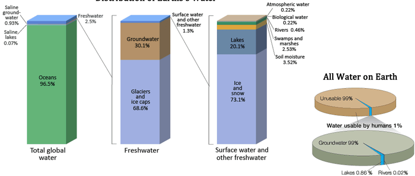
Figure 1. Earth's Water Reservoirs. Bar chart distribution of Earth's water including total global water, freshwater, surface water, and other fresh water and pie chart of water usable by humans and sources of usable water. Source: United States Geographical Survey Igor Skiklomanov's chapter "World fresh water resources" in Peter H. Gleick (editor), 1993, Water in Crisis: A Guide to the World's Fresh Water Resources
