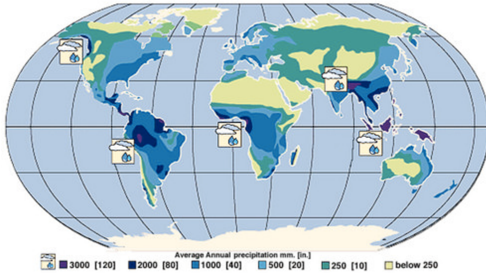
Figure 3. World Rainfall Map. The false-color map above shows the amount of rain that falls worldwide. High rainfall areas include Central and South America, western Africa, and Southeast Asia. Since these areas receive so much rainfall, they are where most of the world's rainforests grow. Areas with very little rainfall usually turn into deserts. The desert areas include North Africa, the Middle East, western North America, and Central Asia. Source: United States Geological Survey Earth Forum, Houston Museum Natural Science
