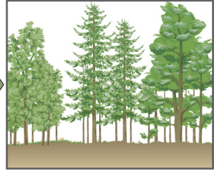
Climax community The mature oak and hickory forest remains stable until the next disturbance.
