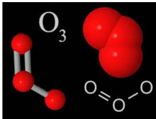
Figure 1. The ozone molecule is comprised of three oxygen atoms covalently bonded. “Ozone” by UCAR (Randy Russell) is licensed under CC BY-SA
