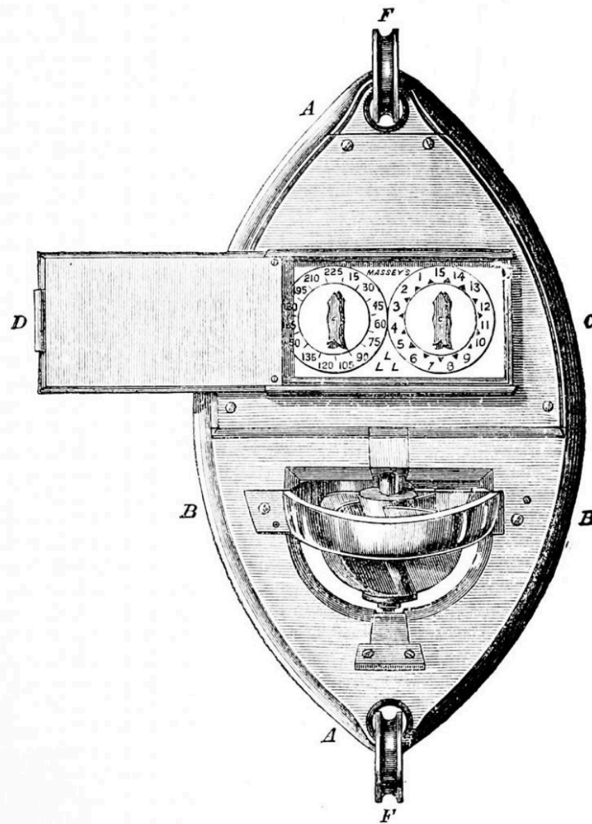
Figure 1.4.2 Massey's sounding machine (Public domain, via Wikimedia Commons).
