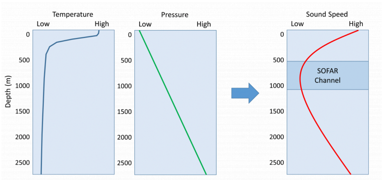
Figure 6.4.1 Profiles of temperature, pressure, and sound speed with depth. Sound speed is high at the surface due to the high temperatures, and is high at depth because of the high pressure. At moderate depths lies the SOFAR channel, the region of slowest sound speed (PW).
