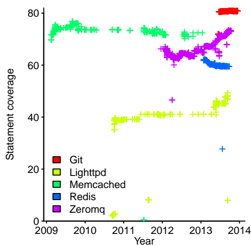
Figure 6.47: Statement coverage achieved by the respective program’s test suite (data on the sixth program was not usable). Data from Marinescu et al. 1207 Github-Local
