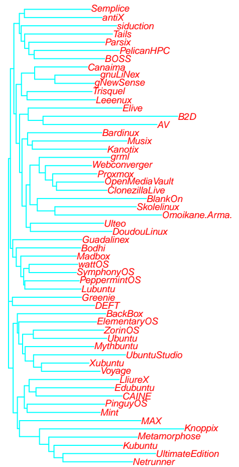
Figure 4.17: Phylogenetic tree of Debian derived distributions, based on which of 50,708 packages are included in each distribution. Data from Keil et al. 984 Github-Local
