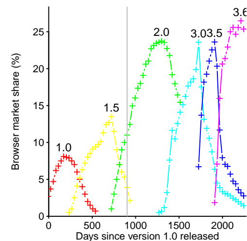
Figure 6.28: Market share of Firefox versions between official release and end-of-support (left of grey line are estimates, right are measurements). Data from Jones. 937 Github-Local
