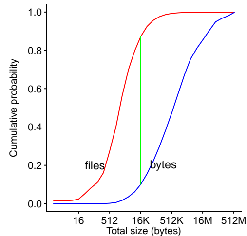
Figure 9.19: Cumulative probability distribution of files size (red) and of number of bytes occupied in a file system (blue). Data from Irlam. 896 Github-Local
