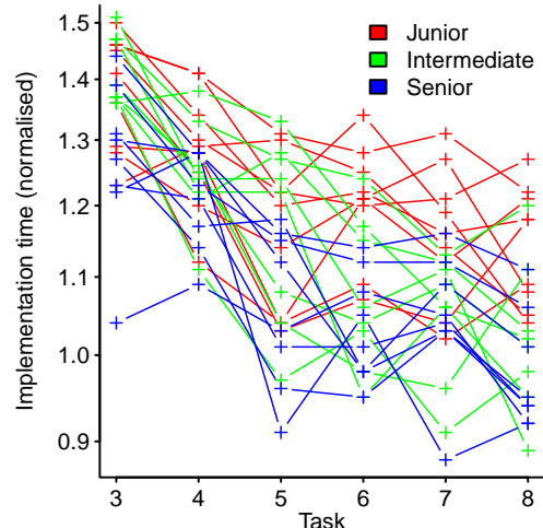
Figure 2.39: Time taken by 24 subjects, classified by years of professional experience, to complete successive tasks. Data from Latorre. 1092 Github-Local
