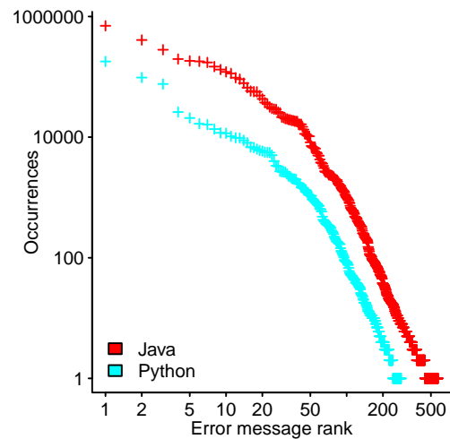
Figure 6.33: Ranked occurrences of compiler messages generated by student submitted Java and Python programs. Data from Pritchard. 1531 Github-Local
