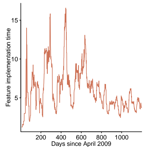
Figure 5.42: Average number of days taken to implement a feature, over time; smoothed using a 25-day rolling mean. Data kindly supplied by 7Digital. 1 Github-Local
