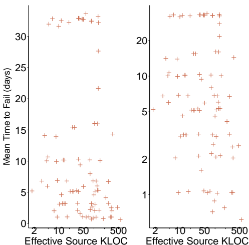
Figure 8.40: Mean time to fail for systems of various sizes (measured in lines of code); linear y-axis left, log y-axis right. Data extracted from Figure 8.3 of Putnam et al. 1538 Github-Local
