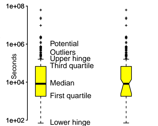
Figure 8.20: Boxplot of time between a potential mistake in Eclipse being reported and the first response to the report; right plot is notched. Data from Breu et al. 252 Github-Local
