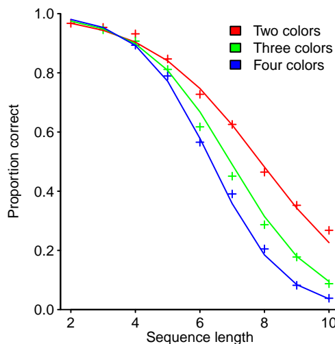
Figure 2.28: Proportion of correctly recalled colored dot sequences of a given length, containing a given number of colors; lines are fitted regression models. Data kindly provided by Chekaf. 341 Github-Local
