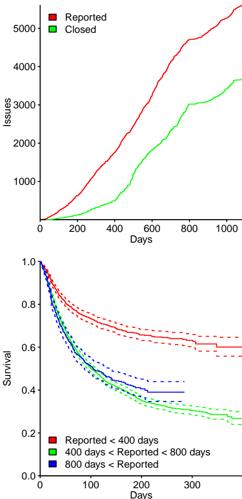
Figure 11.79: Cumulative number of issues reported and closed, and issue survival curves for three intervals. Data from Lunesu. 1172 Github-Local
