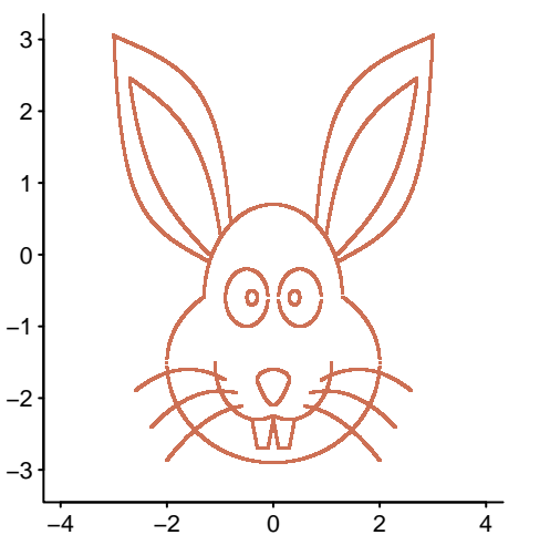
Figure 8.41: What's up doc? Perhaps, not the expected pattern in the data. Equations from White. 1946 Github-Local
