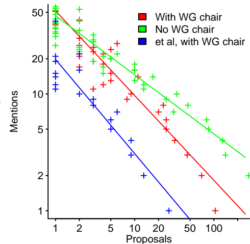
Figure 3.18: Number of proposals receiving a given number of mentions in emails; lines are a fitted regression models of the form: Mentions \propto Proposals^{-a} , where a is 0.51, 0.71, and 0.81. Data from Simcoe et al. 1708 Github-Local
