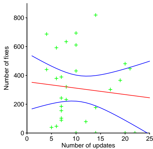
Figure 11.4: Number of updates and fixes in each Linux release between version 2.6.11 and 3.2. Data from Corbet et al. 402 Github-Local
