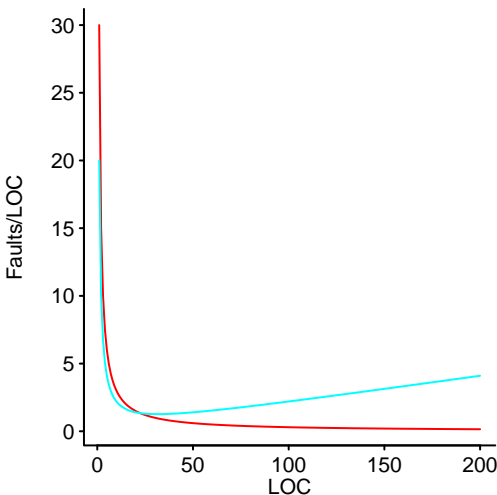
Figure 8.39: Example of U-shape created when y-axis values are a ratio calculated from x-axis values. Github-Local
