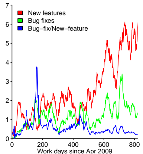
Figure 5.43: Number of feature developments started on a given work day (red new features, green bugs fixes, blue ratio of two values; 25-day rolling mean). Data kindly supplied by 7Digital. 1 Github-Local
