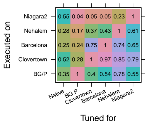
Figure 13.4: Relative performance (y-axis) of libraries optimized to run on various processors (x-axis). Data from Bird. 201 Github-Local
