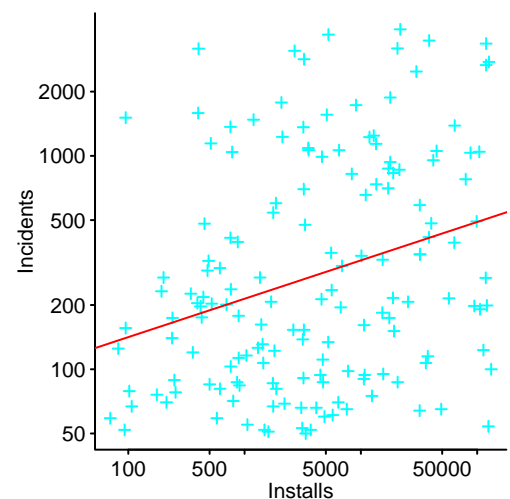
Figure 6.12: Number of incidents reported for each of 800 applications installed on over 120,000 desktop machines; line is fitted regression model. Data from Lucente. 1165 Github-Local
