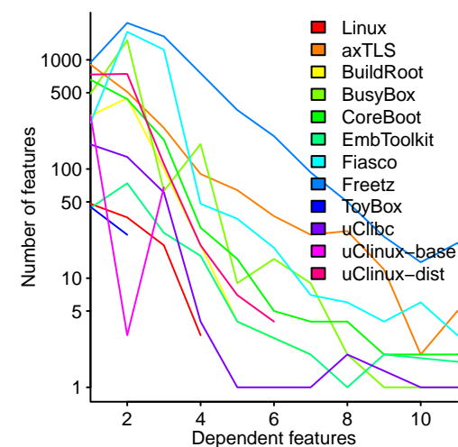
Figure 5.48: Number of optional features selected by a given number of flags. Data kindly provided by Berger. 180 Github-Local
