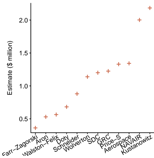
Figure 5.18: Estimated project cost from 12 estimating models. Data from Mohanty. 1304 Github-Local
