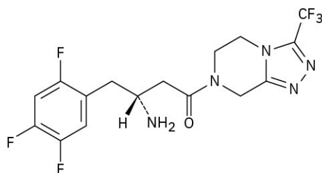
Sitagliptin (Januvia)
