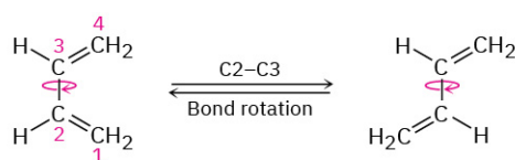
s-Cis conformation
