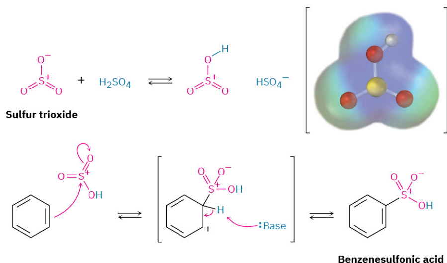
FIGURE 16.6 The mechanism for electrophilic sulfonation of an aromatic ring. An electrostatic potential map of the reactive electrophile \text{HOSO}_2^+ shows that sulfur and hydrogen are the most positive atoms .
