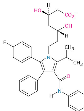
Atorvastatin (Lipitor)
