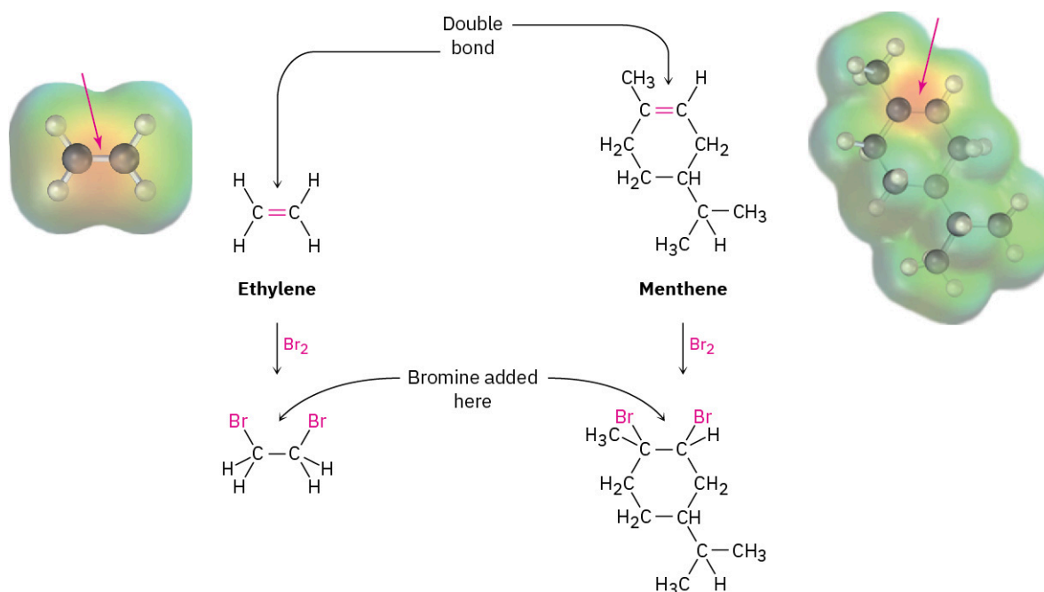
FIGURE 3.2 The reactions of ethylene and menthene with bromine. In both molecules, the carbon–carbon double-bond functional group has a similar polarity pattern, so both molecules react with Br 2 in the same way. The size and complexity of the molecules are not important.
