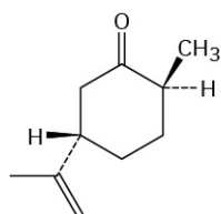
Dihydrocarvone
