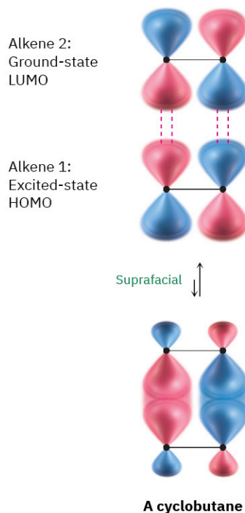
FIGURE 30.11 (a) Interaction of a ground-state HOMO and a ground-state LUMO in a potential [2 + 2] cycloaddition does not occur thermally because the antarafacial geometry is too strained. (b) Interaction of an excited-state HOMO and a ground-state LUMO in a photochemical [2 + 2] cycloaddition reaction is less strained, however, and occurs with suprafacial geometry.
