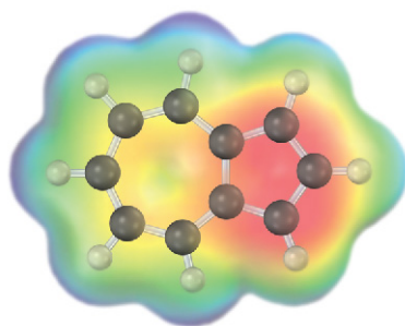
Azulene
