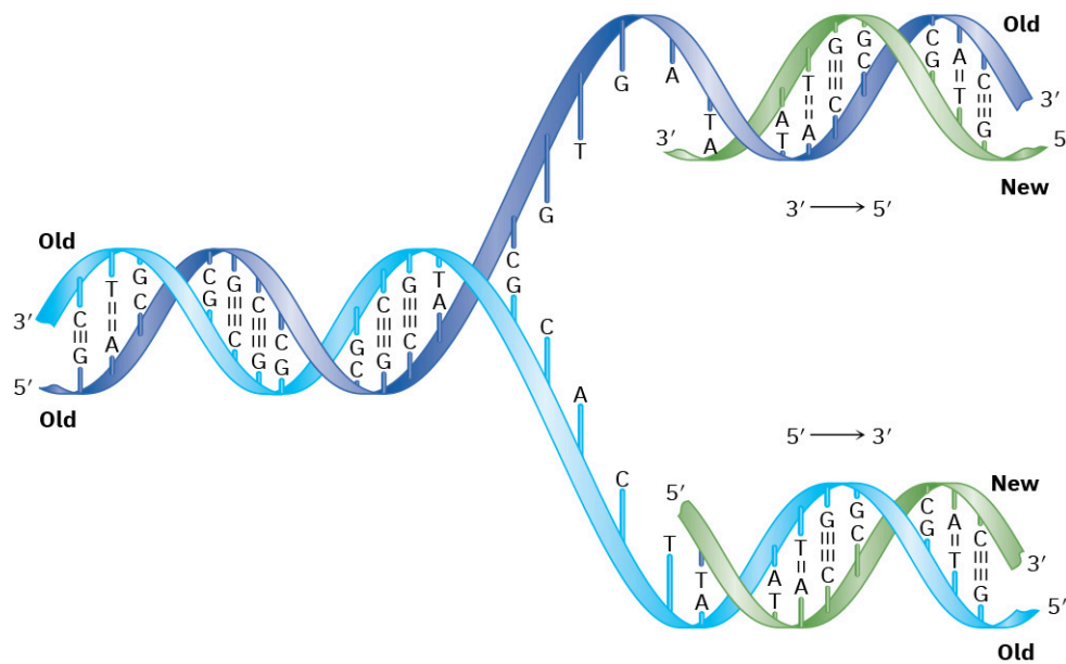
FIGURE 28.5 A representation of semiconservative DNA replication. The original double-stranded DNA partially unwinds, bases are exposed, nucleotides line up on each strand in a complementary manner, and two new strands begin to grow. Both strands are synthesized in the same 5' → 3' direction, one continuously and one in fragments.
