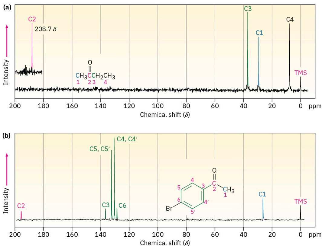
FIGURE 13.19 Carbon- ^{13}\text{C} NMR spectra of (a) 2-butanone and (b) para -bromoacetophenone.
