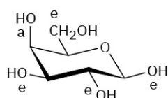
\beta -D-Galactopyranose
