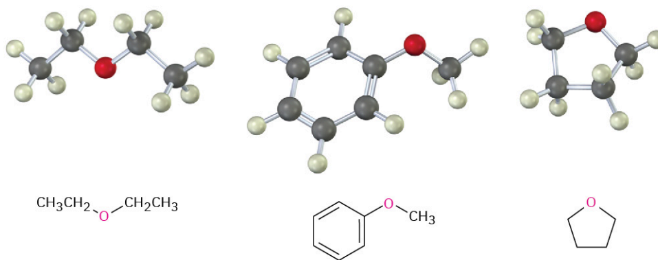
Diethyl ether
