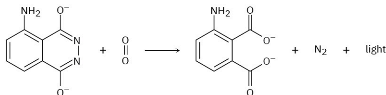
Luminol dianion
