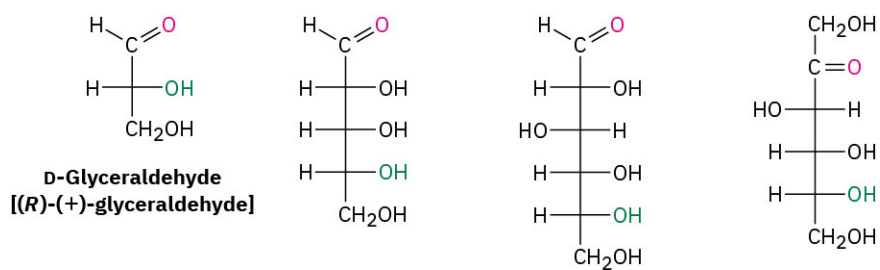
FIGURE 25.3 Some naturally occurring D sugars. The \text{-OH} group at the chirality center farthest from the carbonyl group has the same configuration as (R)-(+)-glyceraldehyde and points toward the right in Fischer projections.
