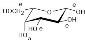
\beta -D-Galactopyranose
