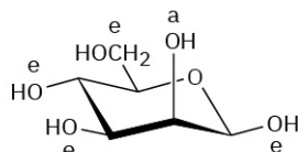
\beta -D-Mannopyranose
