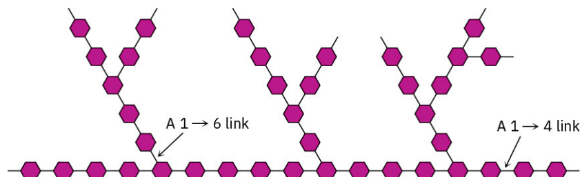
FIGURE 25.12 A representation of the structure of glycogen. The hexagons represent glucose units linked by 1→4 and 1→6 glycoside bonds.
