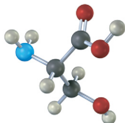
Serine
