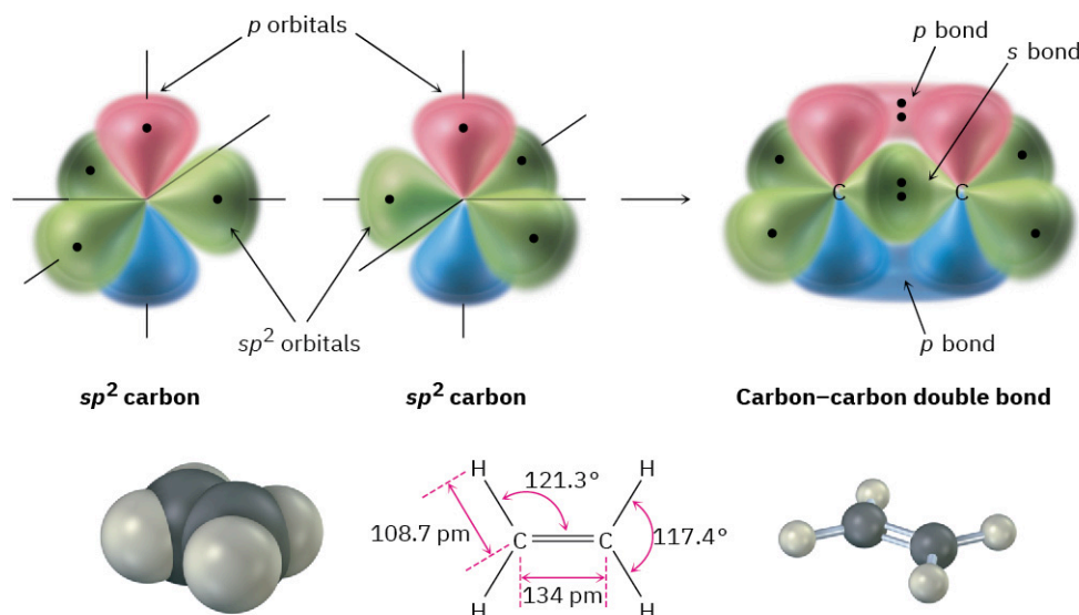
FIGURE 1.15 The structure of ethylene. One part of the double bond in ethylene results from \sigma (head-on) overlap of \text{sp}^2 hybrid orbitals, and the other part results from \pi (sideways) overlap of unhybridized p orbitals (red/blue). The \pi bond has regions of electron density above and below a line drawn between nuclei.
