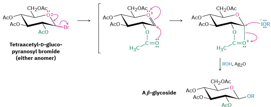
FIGURE 25.7 Mechanism of the Koenigs–Knorr reaction, showing the neighboring-group effect of a nearby acetate.
