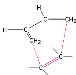
Successful reaction
