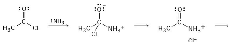
Acetyl chloride
