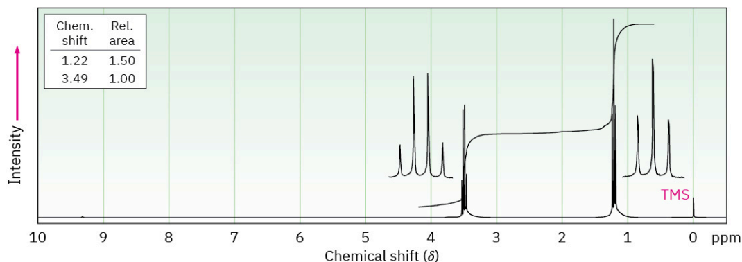
FIGURE 13.12 An integrated ^1\text{H} NMR spectrum for Problem 11.
