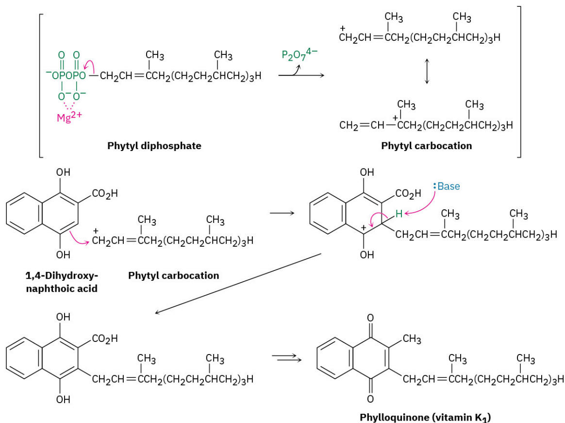
FIGURE 16.11 Biosynthesis of phyloquinone (vitamin \text{K}_1 ) from 1,4-dihydroxynaphthoic acid. The key step that joins the 20-carbon phytyl side chain to the aromatic ring is a Friedel–Crafts-like electrophilic substitution reaction with a diphosphate ion as the leaving group.
