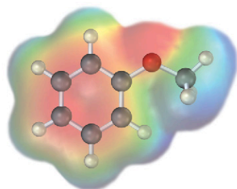
Anisole ( \text{C}_6\text{H}_5\text{OCH}_3 )
