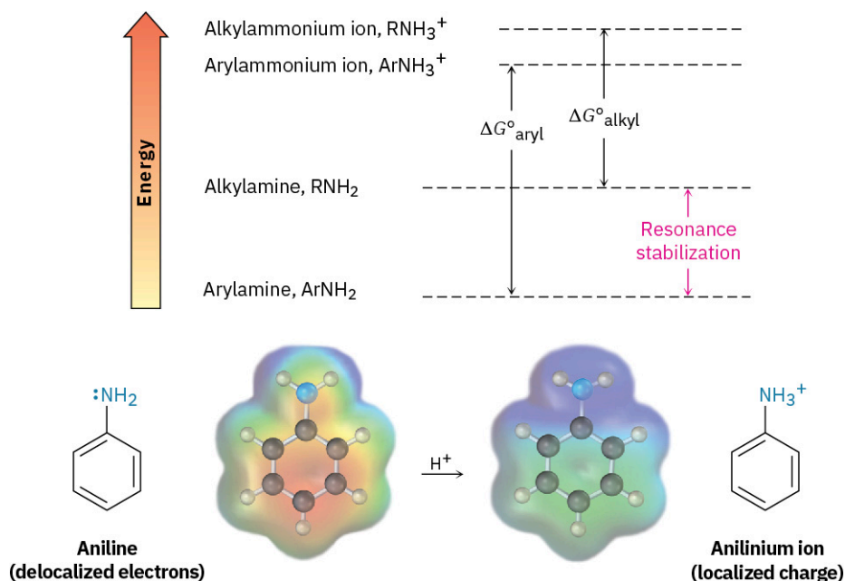
FIGURE 24.5 Arylamines have a larger positive \Delta G^\circ for protonation and are therefore less basic than alkylamines, primarily because of resonance stabilization of the ground state. Electrostatic potential maps show that lone-pair electron density is delocalized in the amine but the charge is localized in the corresponding ammonium ion.
