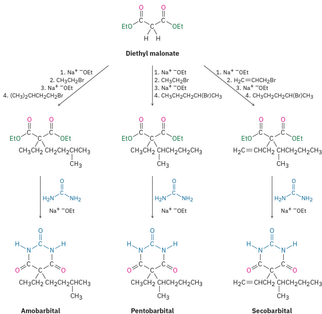
FIGURE 22.9 The synthesis of barbiturates relies on malonic ester alkylations and nucleophilic acyl substitution reactions. More than 2500 different barbiturates have been synthesized over the past 100 years.
