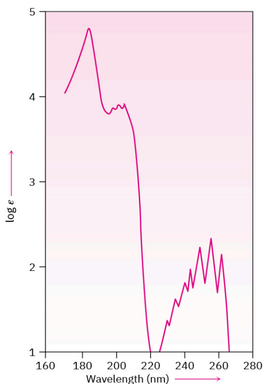
FIGURE 15.13 Ultraviolet spectrum of benzene. There are primary bands at 184 and 202 nm and secondary (fine-structure) bands at 255 nm.
