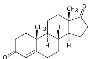
4-Androstene-3,17-dione
