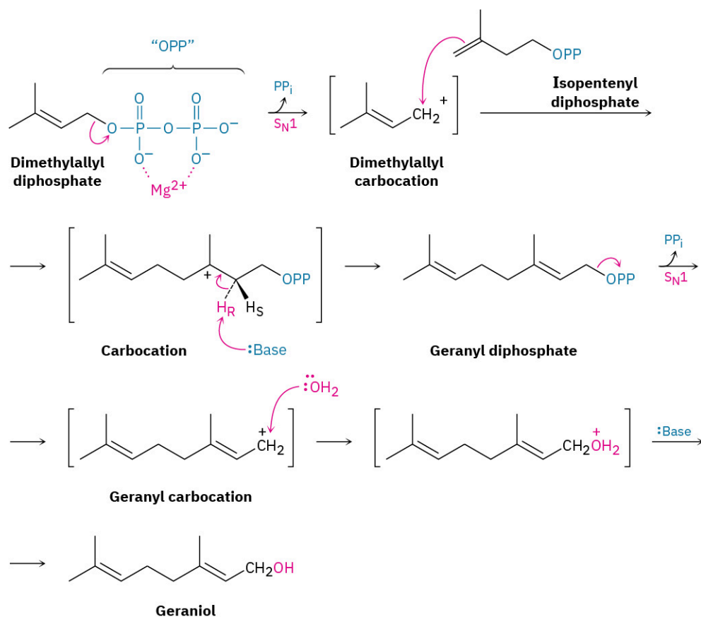
FIGURE 11.16 Biosynthesis of geraniol from dimethylallyl diphosphate. Two \text{S}_{\text{N}}1 reactions occur, both with diphosphate ion as the leaving group.
