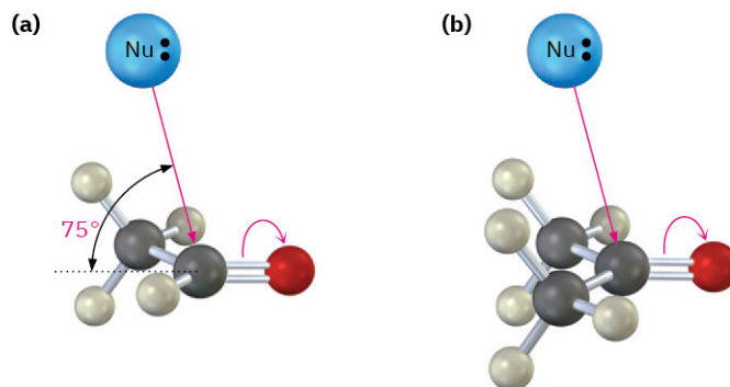
FIGURE 19.4 Steric hindrance in nucleophilic addition reactions. (a) Nucleophilic addition to an aldehyde is sterically less hindered because only one relatively large substituent is attached to the carbonyl-group carbon. (b) A ketone, however, has two large substituents and is more hindered. The approach of the nucleophile is along the C=O bond at an angle of about 75° to the plane of the carbon sp^2 orbitals.
