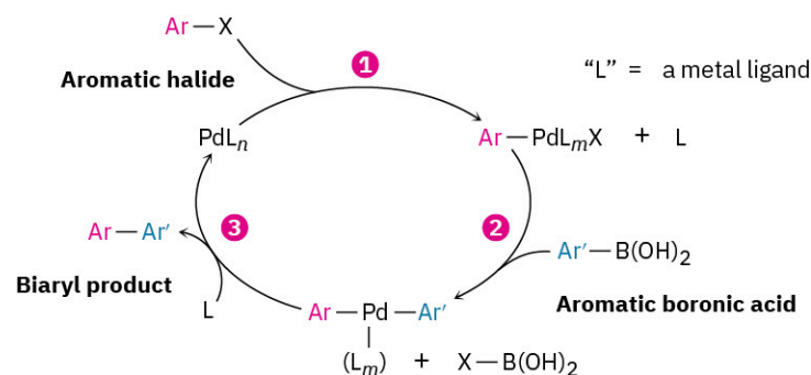
FIGURE 10.6 Mechanism of the Suzuki–Miyaura coupling reaction of an aromatic boronic acid with an aromatic halide to give a biaryl. The reaction takes place by (1) reaction of the aromatic halide, \text{ArX} , with the catalyst to form an organopalladium intermediate, followed by (2) reaction with the aromatic boronic acid. (3) Subsequent decomposition of the diarylpalladium intermediate gives the biaryl product.
