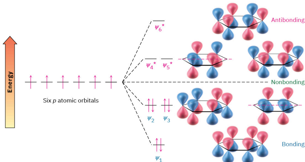
Six benzene molecular orbitals
