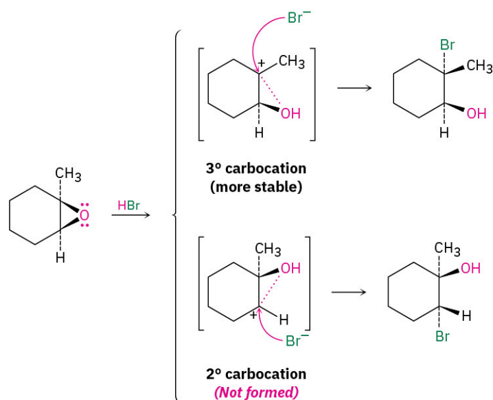
FIGURE 18.2 Ring-opening of 1,2-epoxy-1-methylcyclohexane with HBr. There is a high degree of \text{S}_{\text{N}}1 -like carbocation character in the transition state, which leads to backside attack of the nucleophile at the tertiary center and to formation of a product isomer that has -\text{Br} and -\text{OH} groups trans.
