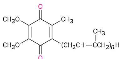
Ubiquinones ( n = 1-10 )
