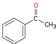
Acetophenone
