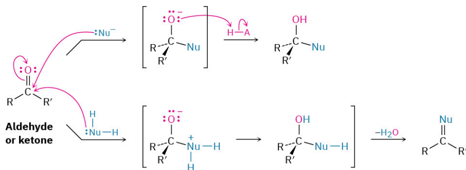
FIGURE 18.9 The addition reaction of an aldehyde or a ketone with a nucleophile. Depending on the nucleophile, either an alcohol or a compound with a C=Nu double bond is formed.
