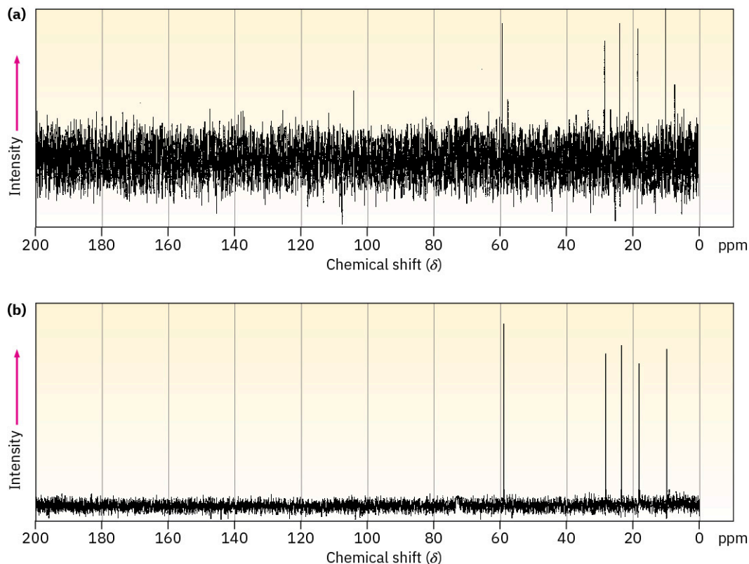
FIGURE 13.17 Carbon- ^{13}\text{C} NMR spectra of 1-pentanol, \text{CH}_3\text{CH}_2\text{CH}_2\text{CH}_2\text{CH}_2\text{OH} . Spectrum (a) is a single run, showing the large amount of background noise. Spectrum (b) is an average of 200 runs.
