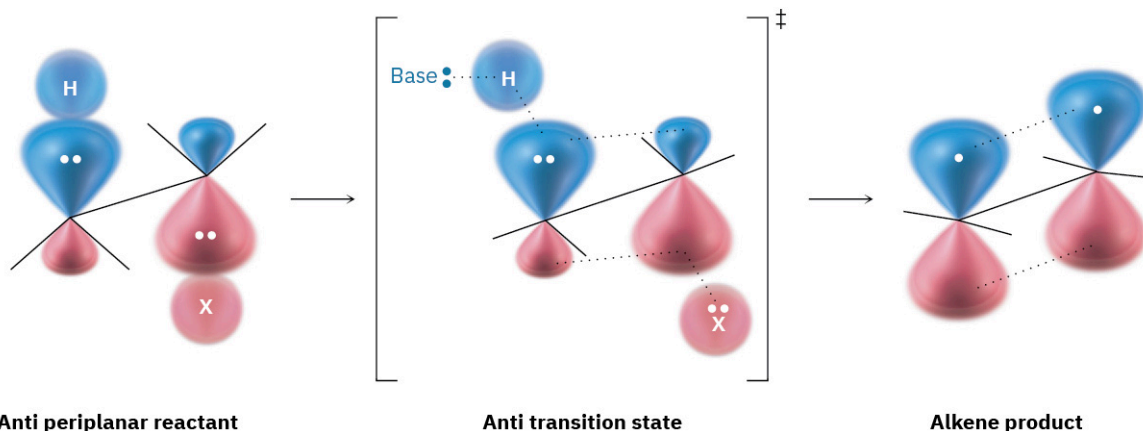
FIGURE 11.19 The transition state for the E2 reaction of an alkyl halide with base. Overlap of the developing p orbitals in the transition state requires periplanar geometry of the reactant.
