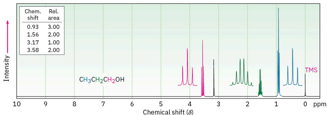
FIGURE 17.14 ^1\text{H} NMR spectrum of 1-propanol. The protons on the oxygen-bearing carbon are split into a triplet at 3.58 \delta .
