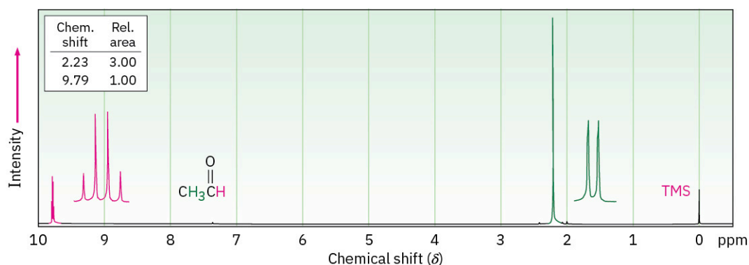
FIGURE 19.16 ^1\text{H} NMR spectrum of acetaldehyde. The absorption of the aldehyde proton appears at 9.79\text{ }\delta and is split into a quartet.
