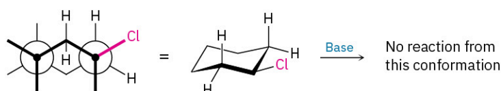
FIGURE 11.20 The geometric requirement for an E2 reaction in a substituted cyclohexane. The leaving group and the hydrogen must both be axial for anti periplanar elimination to occur.
