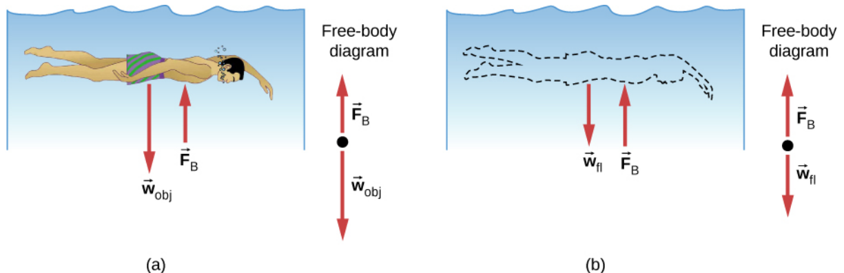
Figure 14.21 (a) An object submerged in a fluid experiences a buoyant force F_B . If F_B is greater than the weight of the object, the object
