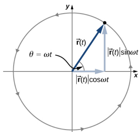
Figure 4.20 The position vector for a particle in circular motion with its components along the x- and y-axes. The particle moves counterclockwise. Angle \theta is the angular frequency \omega in radians per second multiplied by t .
