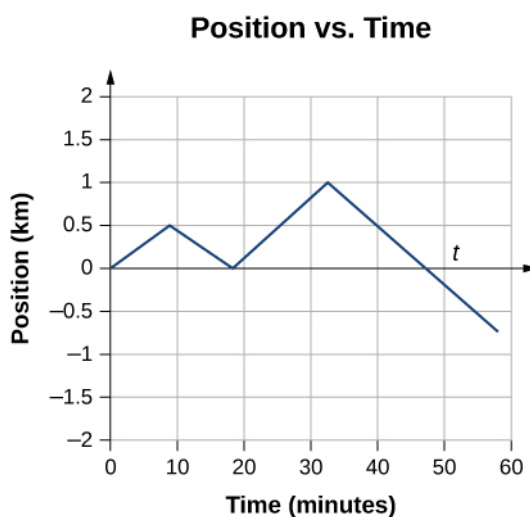
Figure 3.5 This graph depicts Jill's position versus time. The average velocity is the slope of a line connecting the initial and final points.
