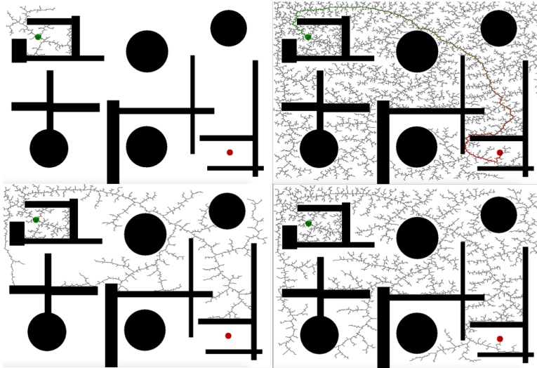
Figure 13.5. Counterclockwise from top-left: Random exploration of a 2D search space by randomly sampling points and connecting them to the graph until a feasible path between start and goal is found.
