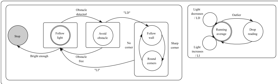
Figure 11.5. A hierarchical FSM with the states from Figure 11.4 as super states, a more sophisticated wall-following behavior, and signal processing for averaging the light measurement being performed in parallel.
