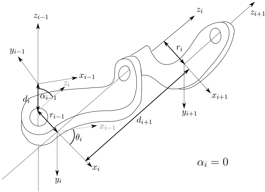
Figure 3.2. Example of selected Denavit-Hartenberg parameters for three sequential revolute joints. The z -axes of joint i and i+1 are parallel, which results in \alpha_i = 0 .
