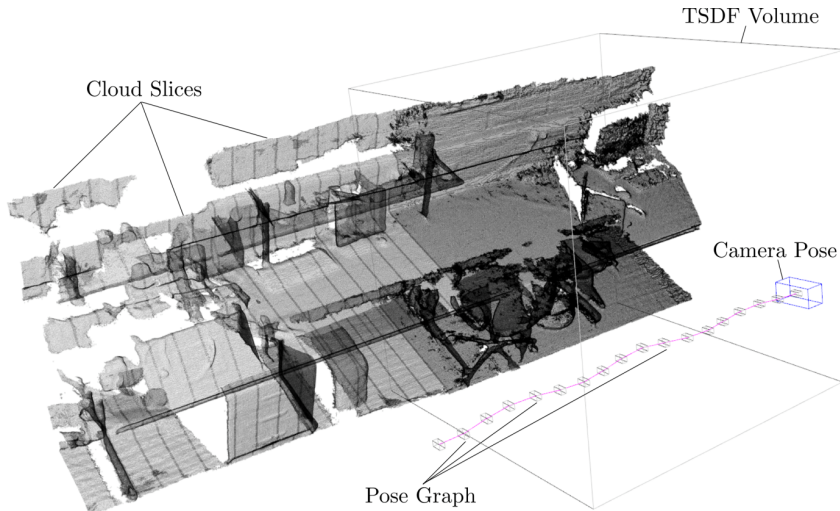
Figure 12.3. Fused point cloud data from a walk through of an office environment using “Kintinuous”. Picture courtesy of John Leonard.
