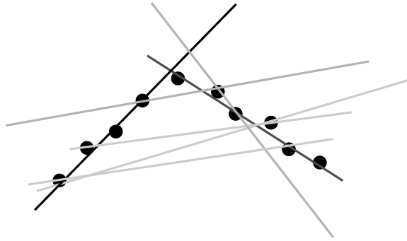
Figure 9.3. Random Sample and Consensus (RANSAC). Random lines are evaluated by counting the number of points close by (“inliers”), darker lines are better fits.
