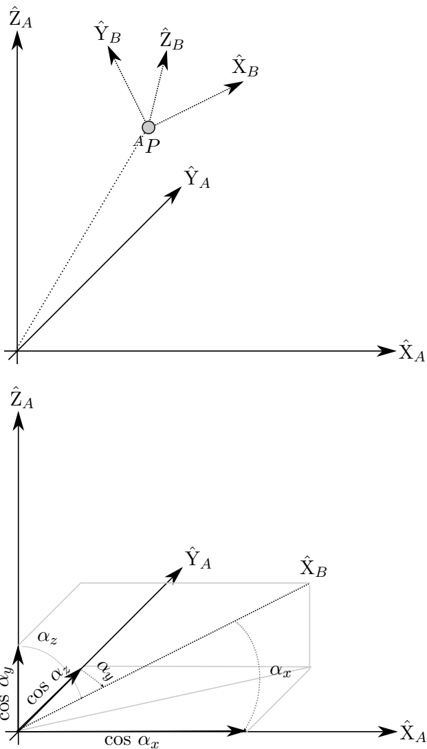
Figure 2.8. Top: A coordinate system \{B\} with position given by {}^A P and orientation given by \hat{X}_B , \hat{Y}_B , and \hat{Z}_B . Bottom: The projection of the unit vector \hat{X}_B onto the unit vectors that span coordinate system \{A\} after moving \{B\} into the origin of \{A\} . As all vectors are unit vectors, A \cdot B = \|A\| \|B\| \cos \alpha = \cos \alpha .
