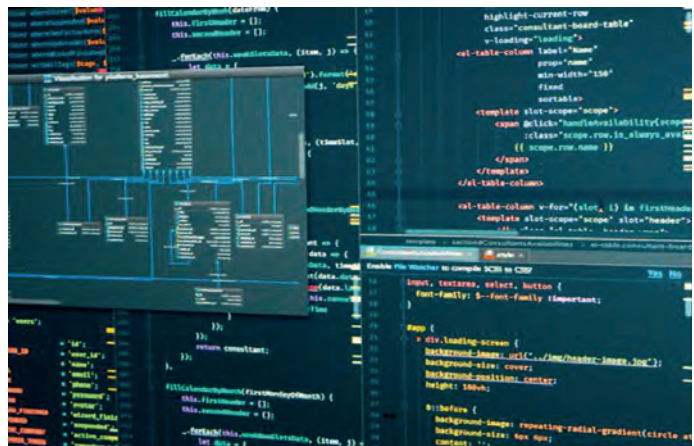
Figure 5.4: Software Troubleshooting
