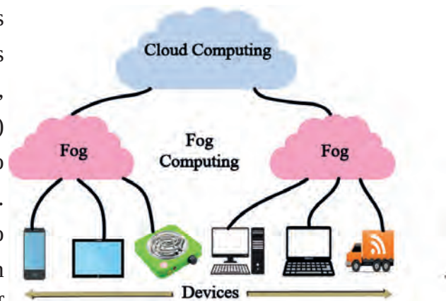
Figure 2.27. Fog Computing
