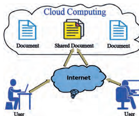
Figure 2.14. Flexibility
