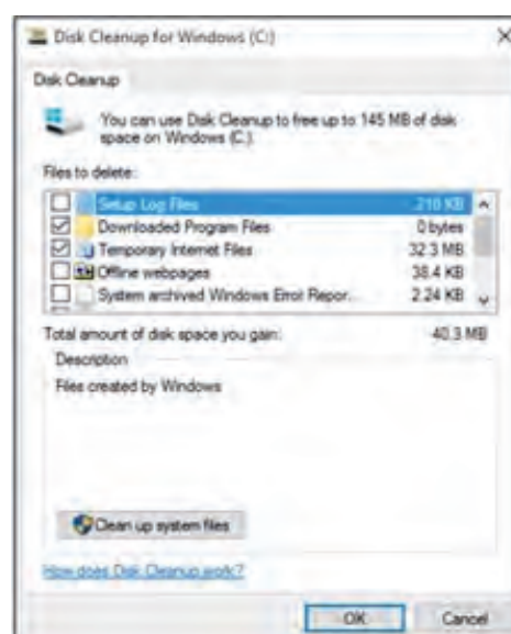
Figure 5.9. Disk Cleanup
