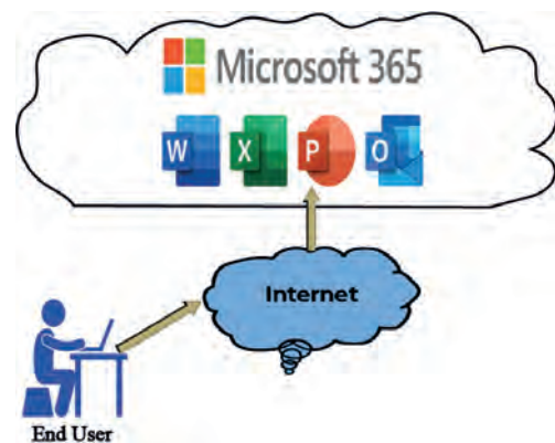
Figure 2.24. Hybrid cloud
