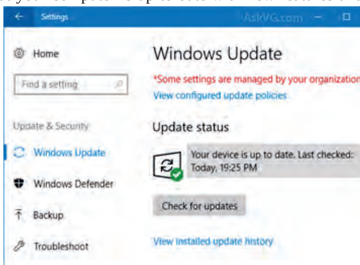
Figure 5.10. Window Update
