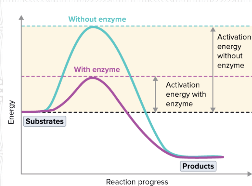
Figure 3.5 Enzymatic reactions between glucose and oxygen
