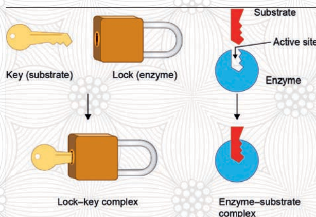
Figure 3.10 Lock and Key model
