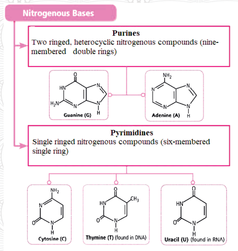
Figure 4.2 Structures of purine and pyrimidine
